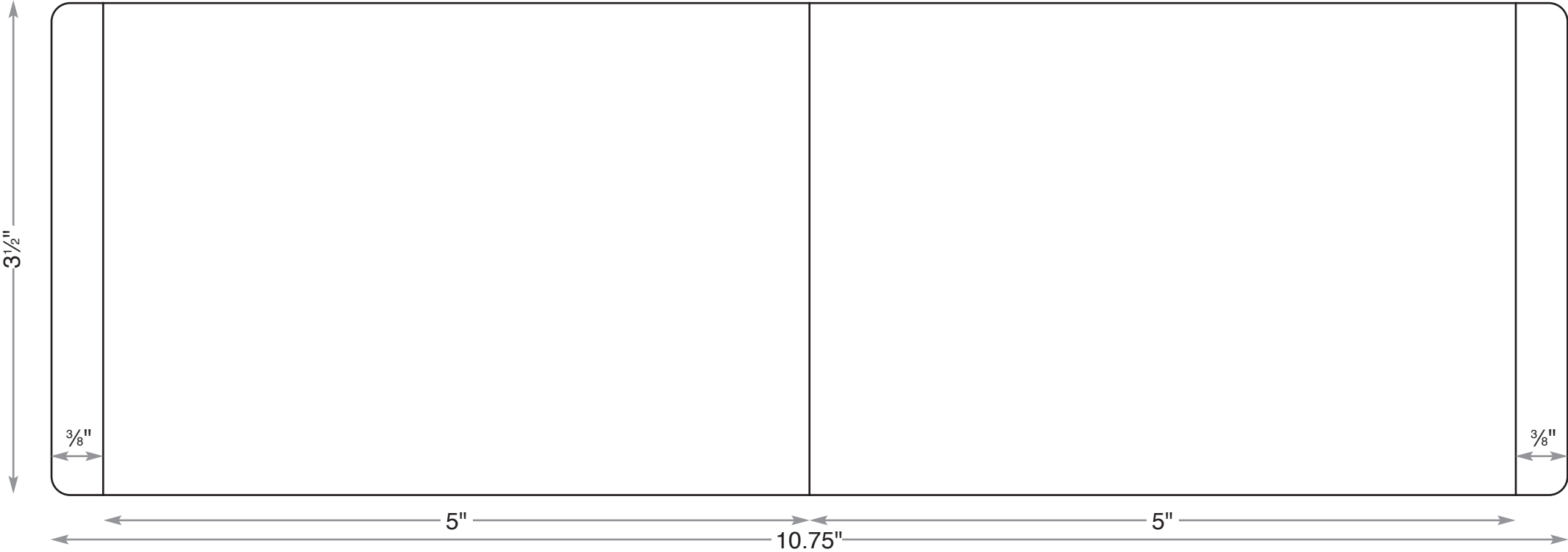
Oversized Magnet Cover – Outside Back
